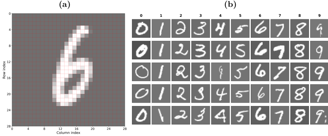
Figure 1. (a) One MNIST digit ( 28 \times 28 ): red lines mark pixel boundaries; row and column indices run from 0 to 28. (b) Reference library: five examples per digit 0–9 after zero-mean and \ell_2 normalization (100 references stored per class in the main experiment).
